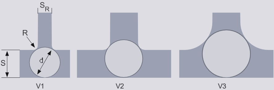
Influence of the rib thickness (S) and the rounding radius (R) on the cooling time.
