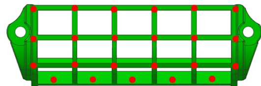
Positioning of the ejectors (DFM Report)
