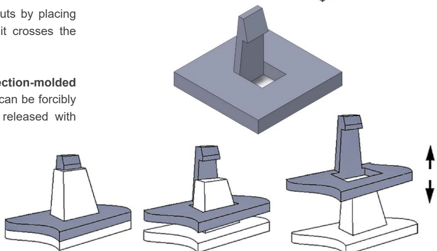
Use of a slider
