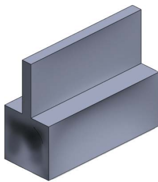
Sinkholes
