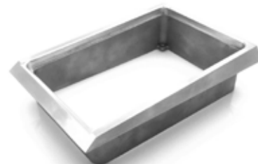
Touchscreen Frame with Brushing Finishing Mat. AISI304L
