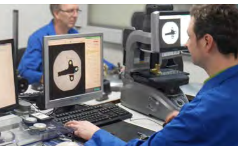
optical measurement with digital measuring projectors
