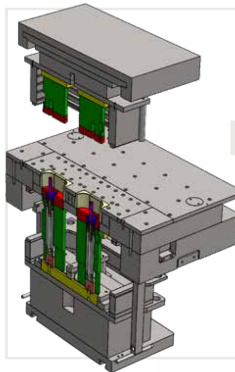
Double cavity mold for sliding plates
